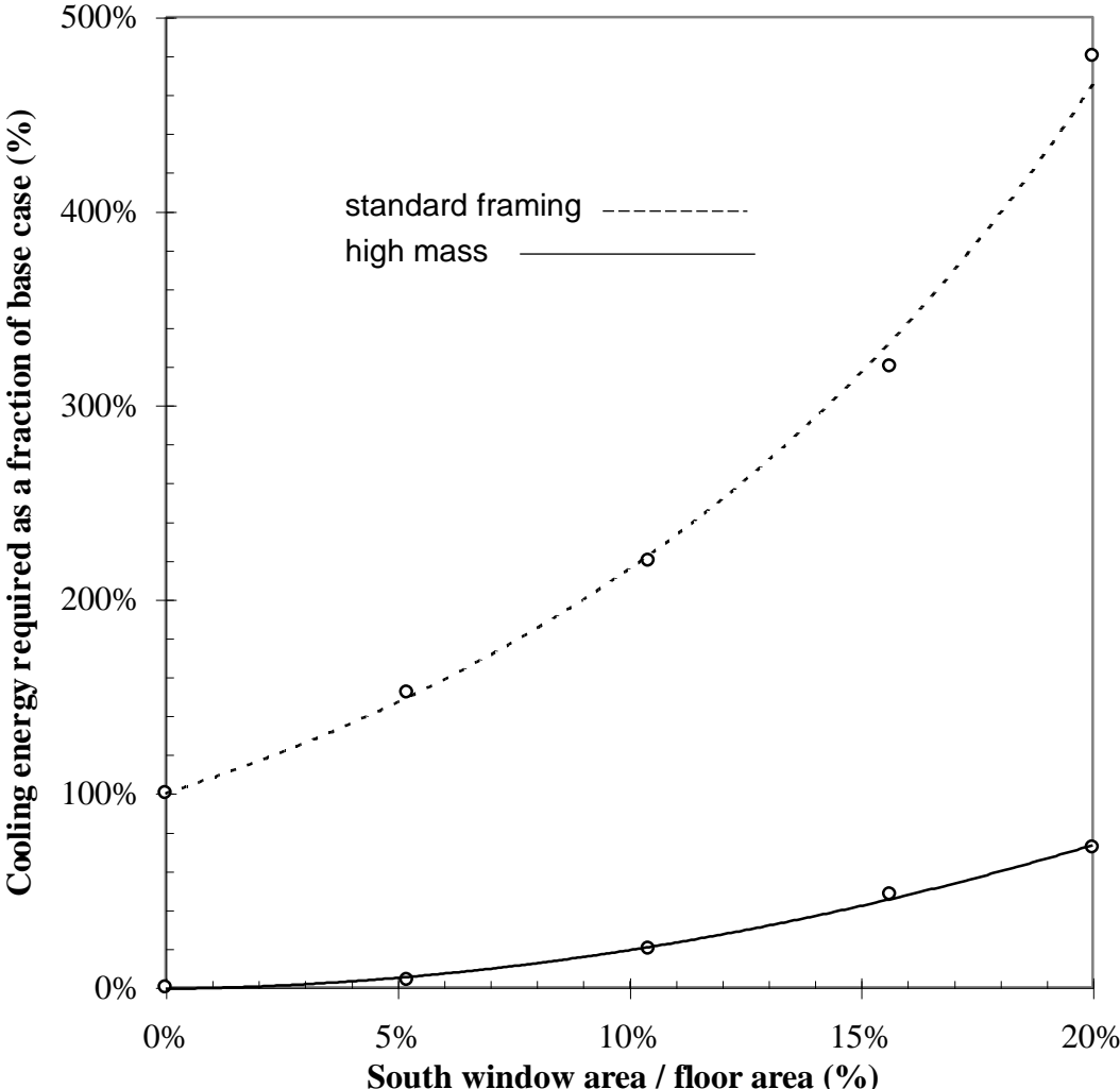
Cooling Energy Savings Due to Mass Effect
